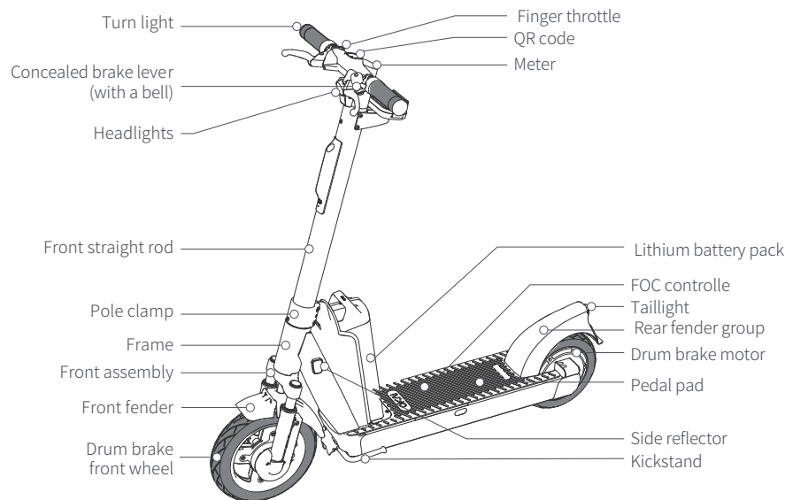
Size:L1247mm*W521mm*H1210mm Figure 1
